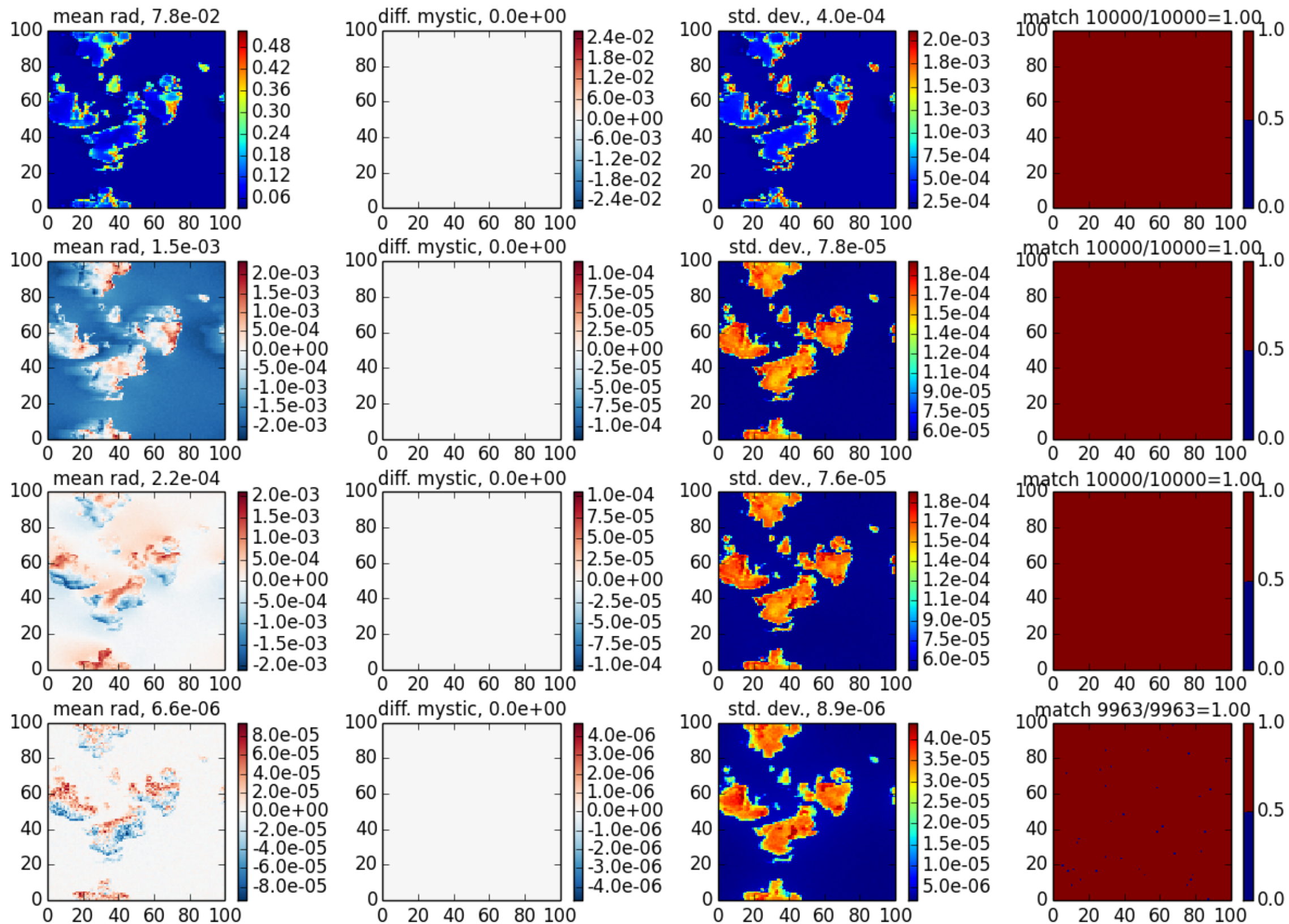
mystic case 4, \theta_0=20 , z=0 , \theta=40 , \phi=180
