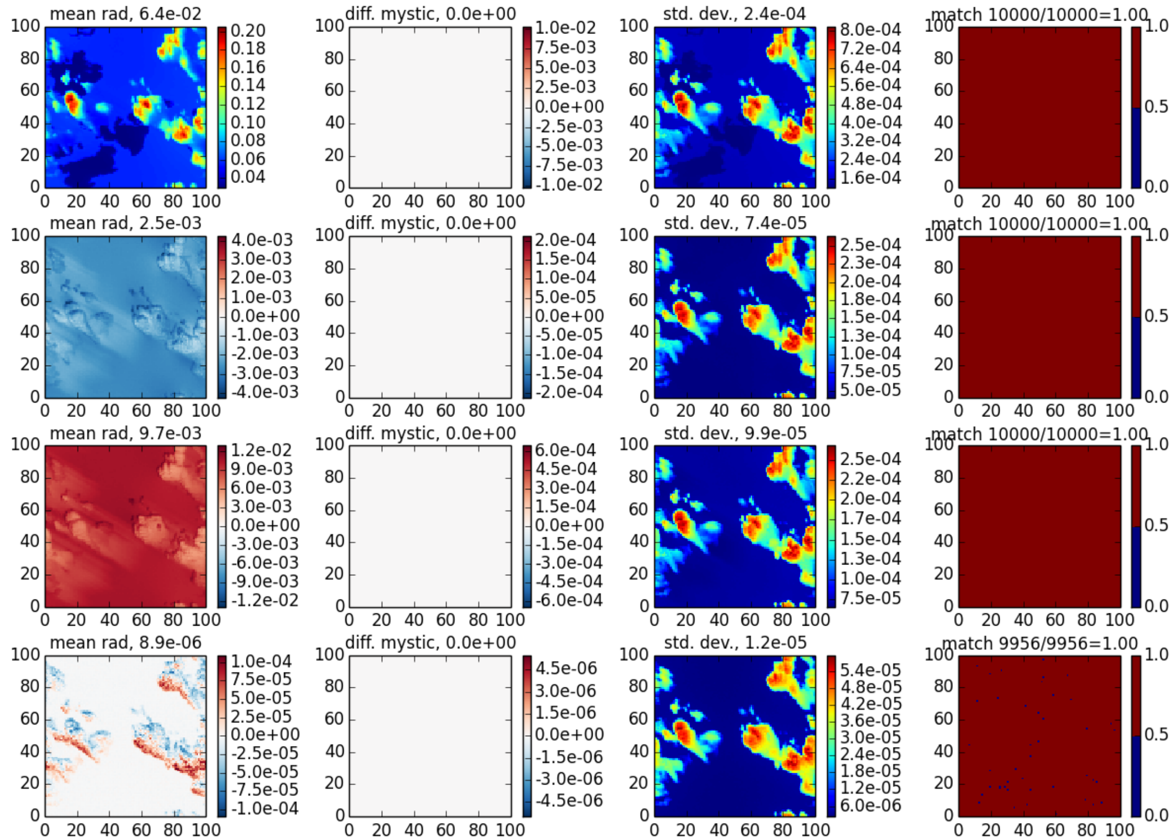
mystic case 8, \theta_0=40 , z=30 , \theta=140 , \phi=120
