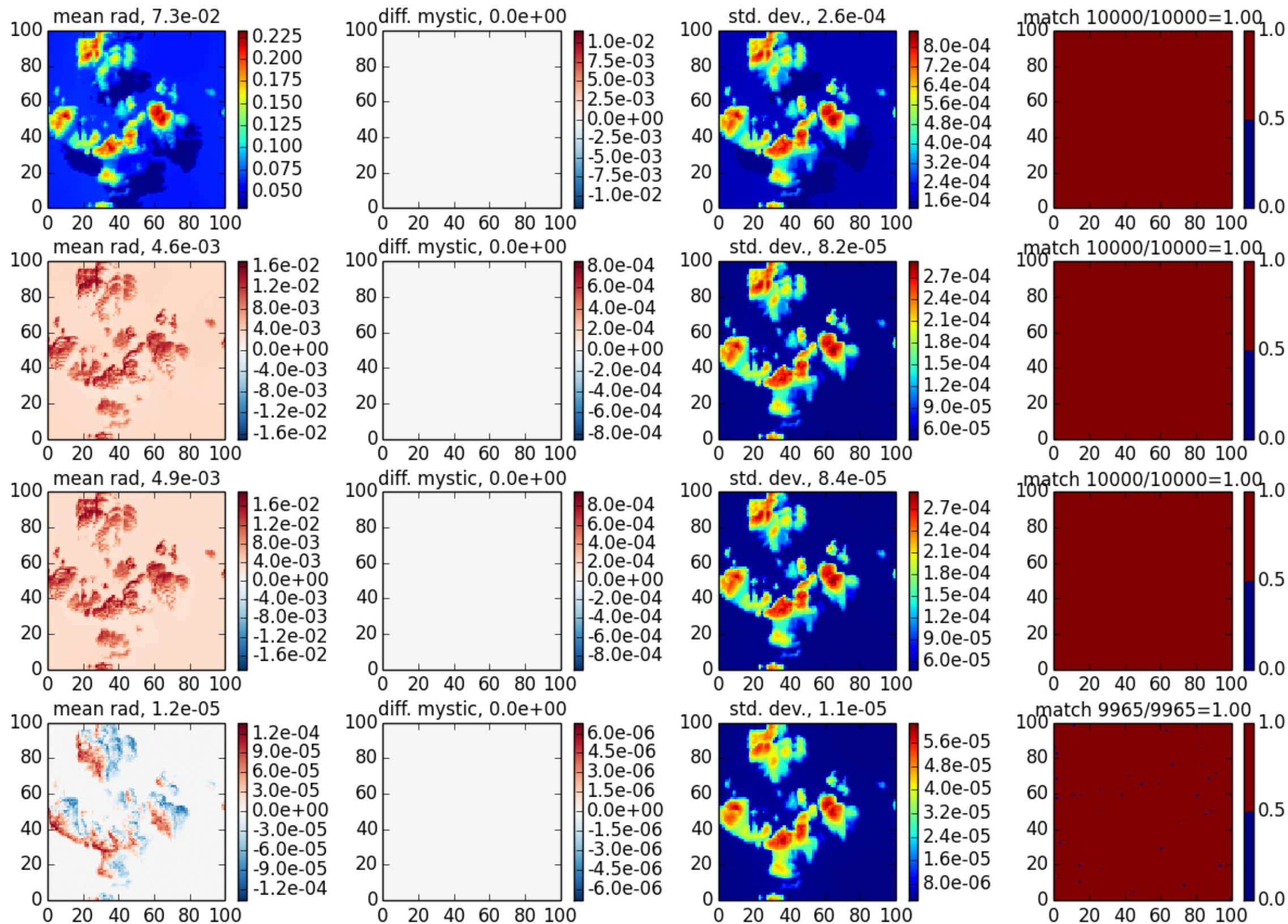
mystic case 7, \theta_0=40 , z=30 , \theta=140 , \phi=60
