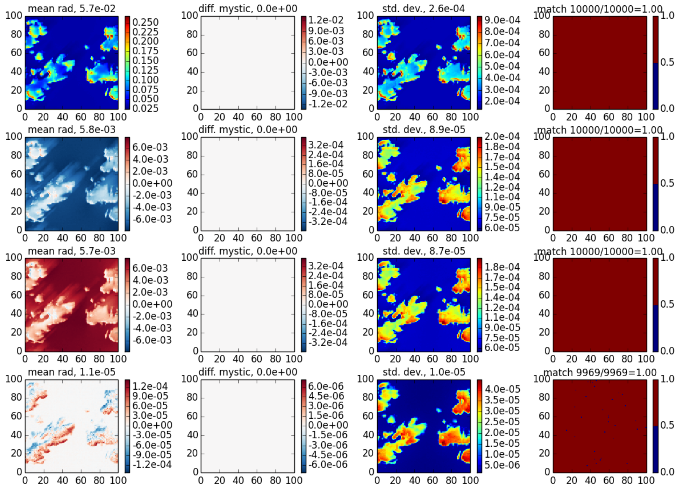
mystic case 2, \theta_0=20 , z=0 , \theta=40 , \phi=60
