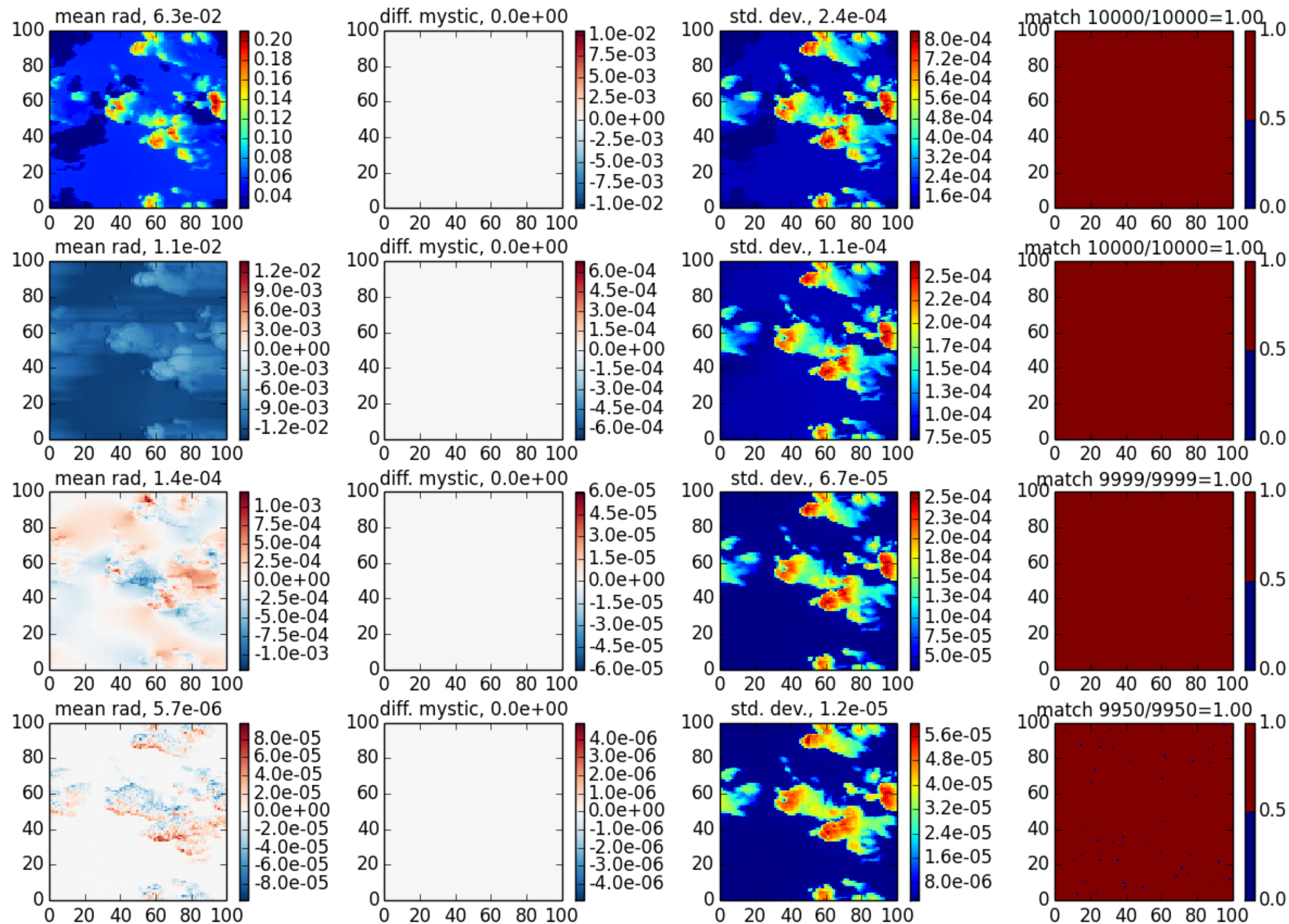
mystic case 9, \theta_0=40 , z=30 , \theta=140 , \phi=180
