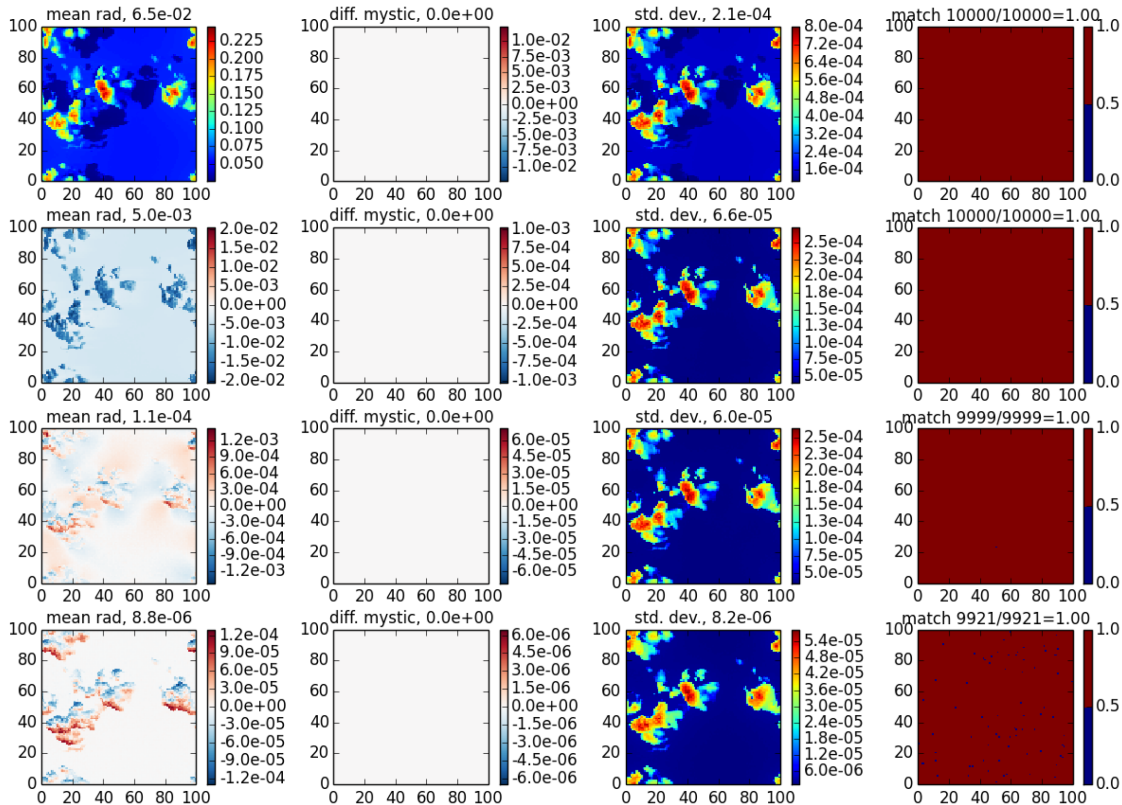
mystic case 5, \theta_0=40 , z=30 , \theta=180 , \phi=0
