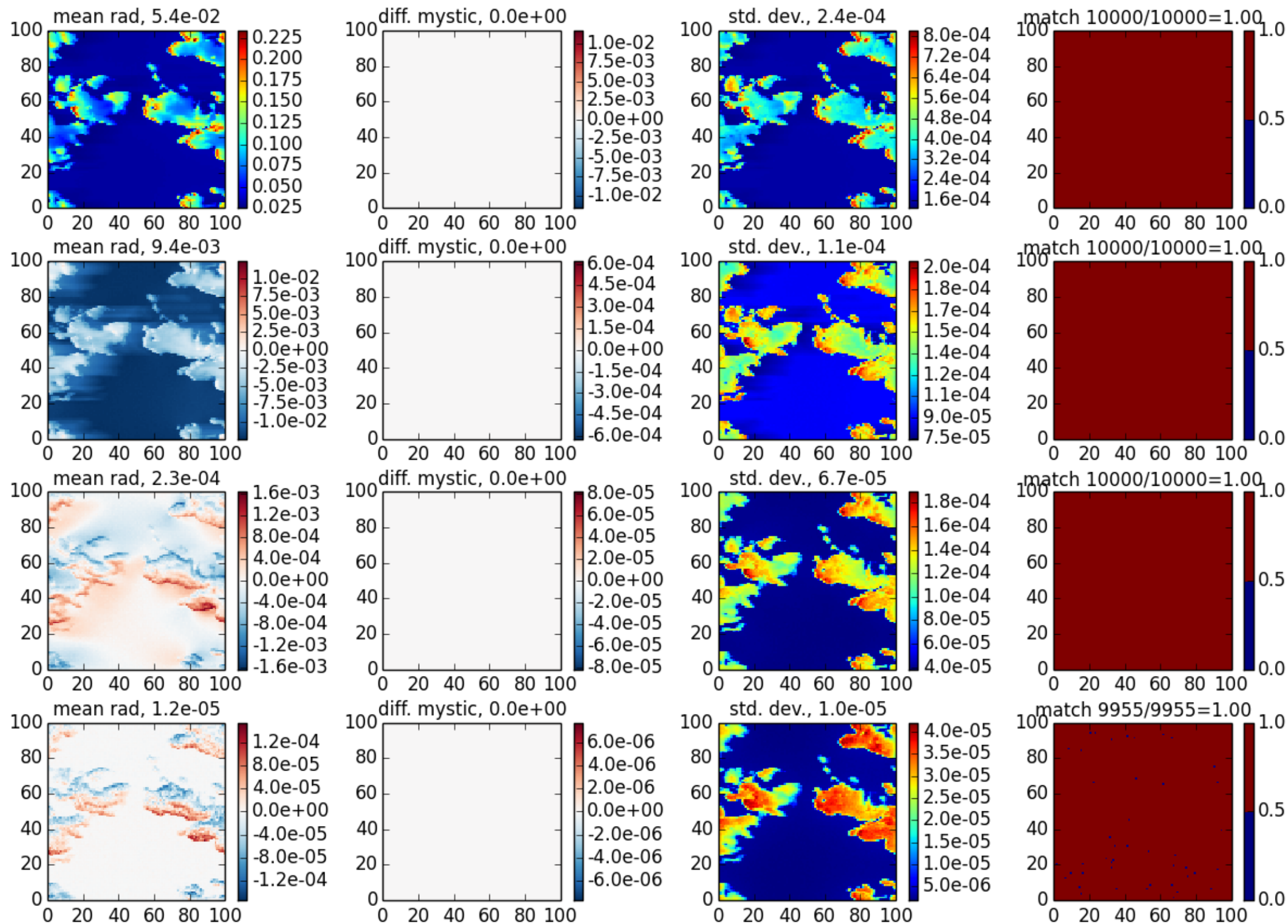
mystic case 1, \theta_0=20 , z=0 , \theta=40 , \phi=0
