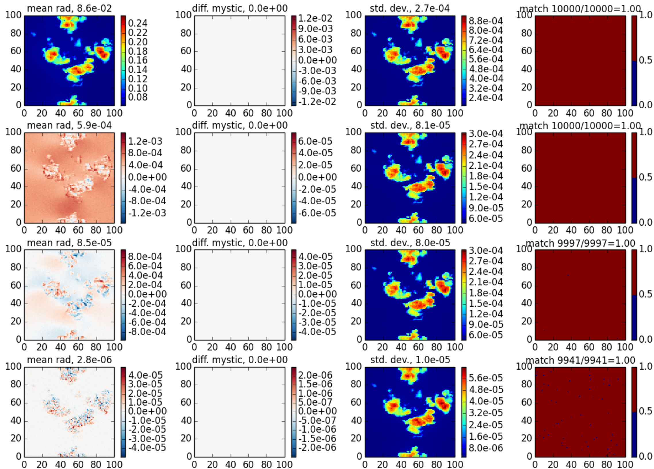
mystic case 6, \theta_0=40 , z=30 , \theta=140 , \phi=0
