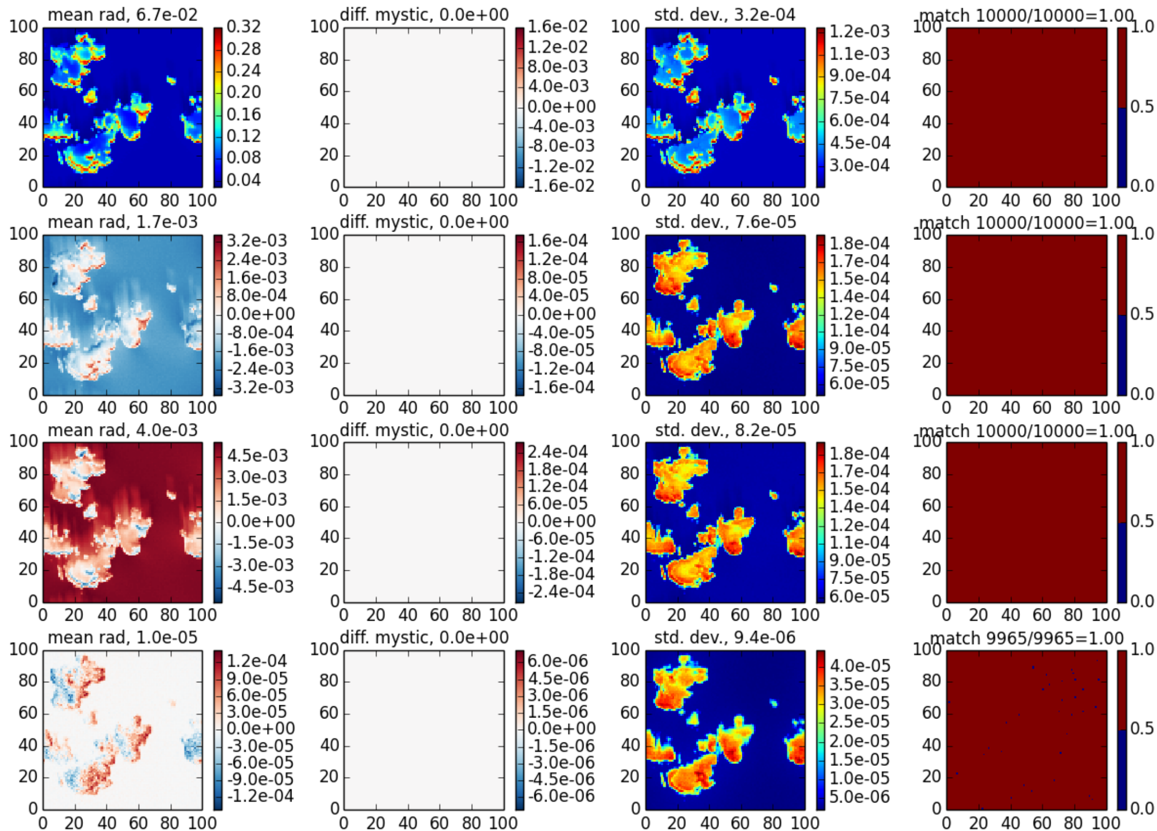
mystic case 3, \theta_0=20 , z=0 , \theta=40 , \phi=120
